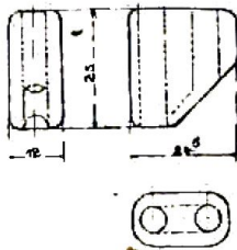
Fig. 52. — Raccord Minet.
